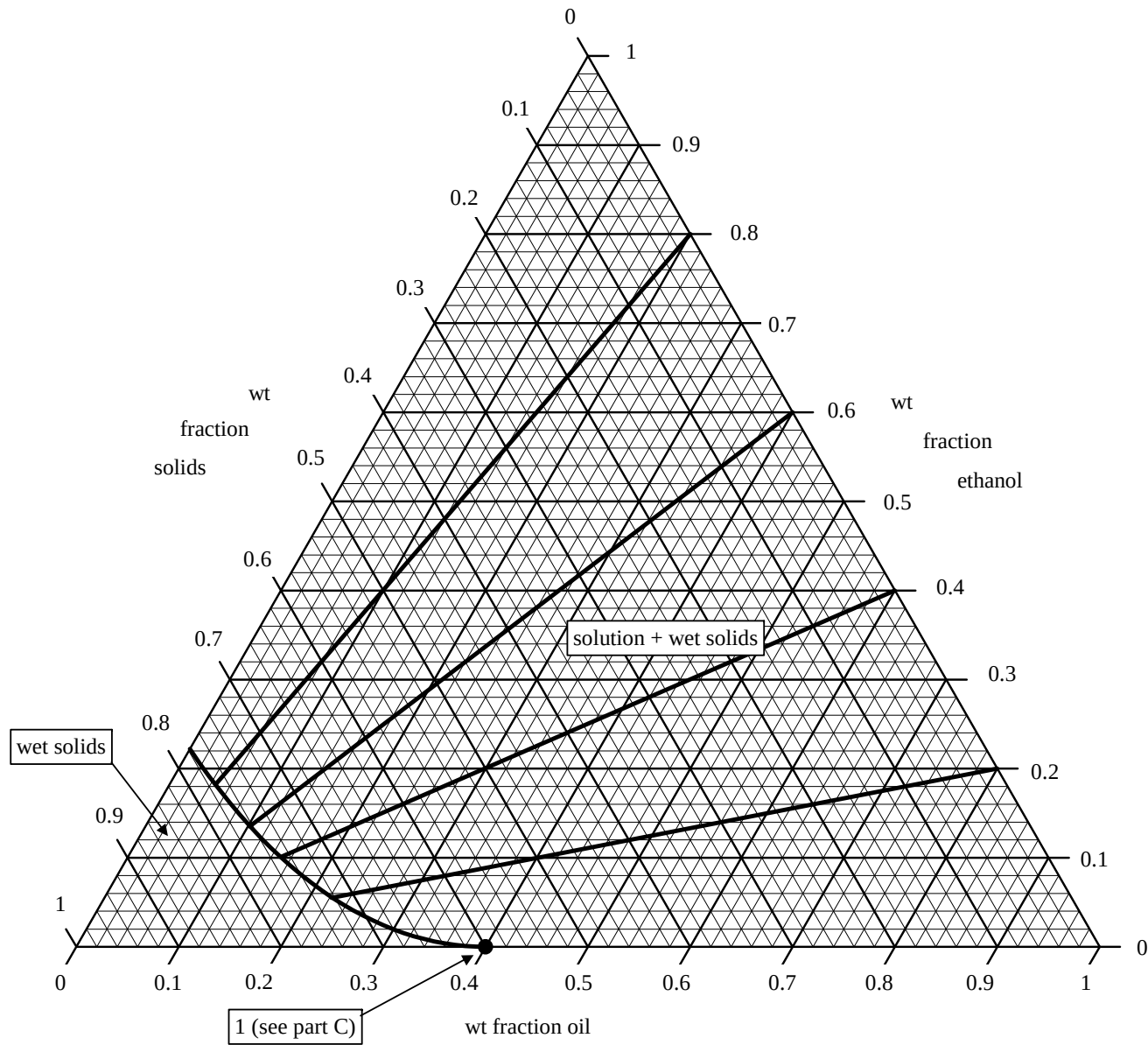
ternary phase diagram for solids - oil - ethanol mixtures
