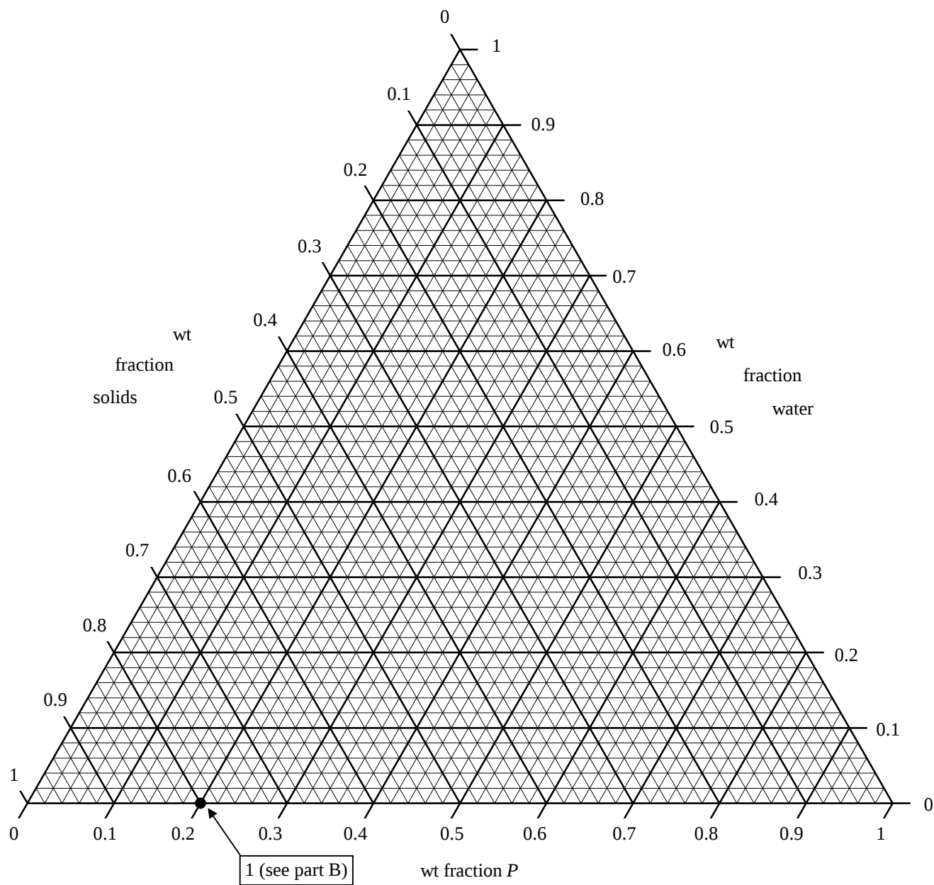
ternary diagram for solids - P (liquid) - water mixtures
