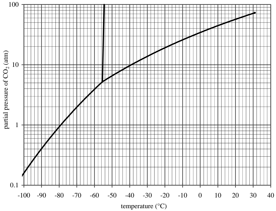
pressure-temperature phase diagram for CO 2
