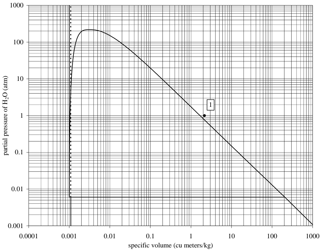
pressure-volume phase diagram for H 2 O
