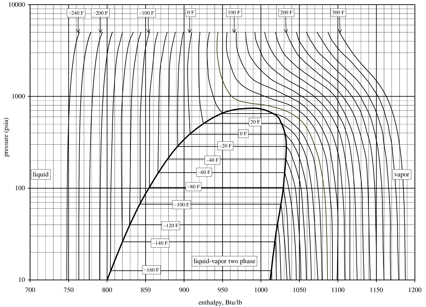
pressure-enthalpy diagram for ethylene
